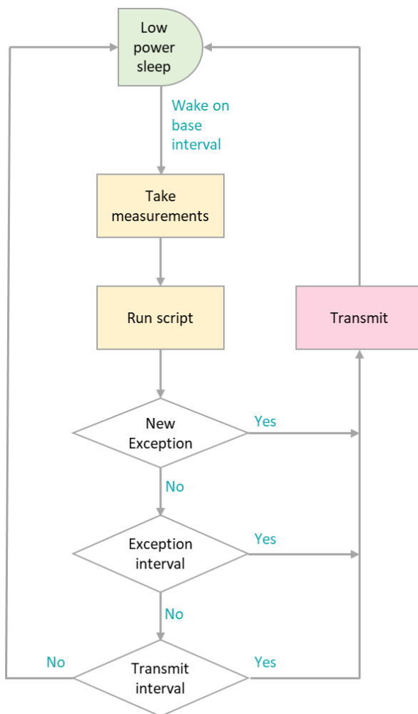
Figure 2 - Simplified Device Flowchart
